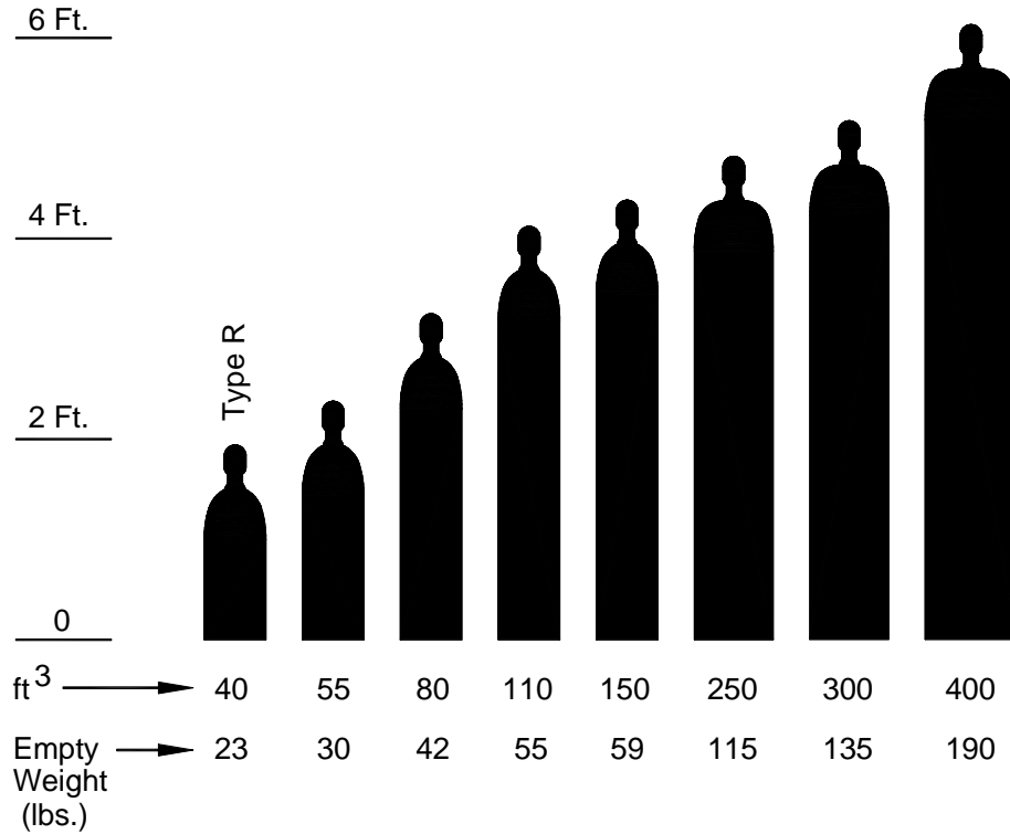
Figure 1. Oxygen cylinder sizes.
